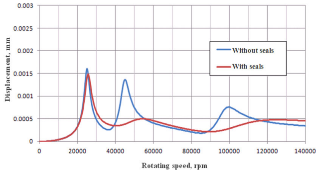
Figure 7. Displacement in section 1 of turbine stage
