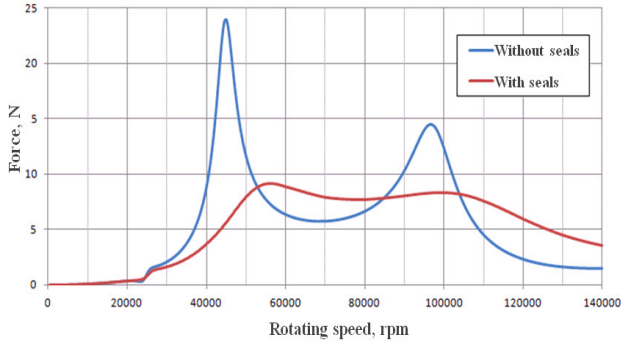
Figure 6. Loads in section elastic-damping support 2
