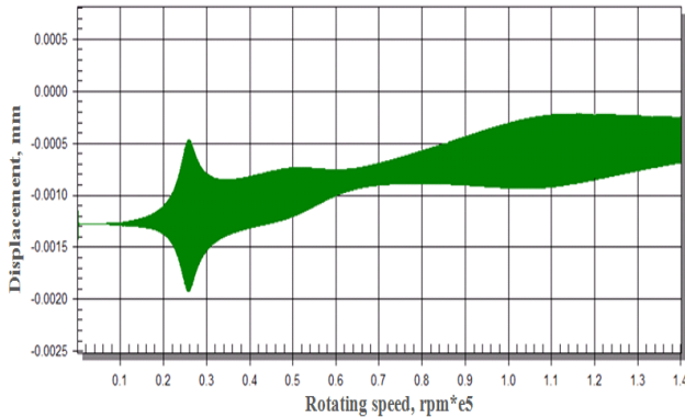
Figure 11. Amplitude-time characteristic of rotor in section of elastic-damping support 1 (unbalance 1 - 0.01 gcm; unbalance 2 - 0.01 gcm)
