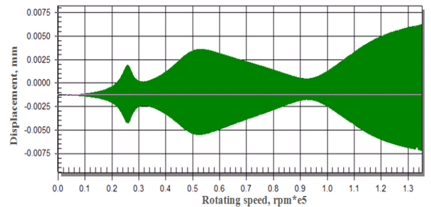
Figure 14. Amplitude-time characteristic of rotor in section of elastic-damping support 1 (unbalance 1 - 0.05 gcm; unbalance 2 - 0.05 gcm)
