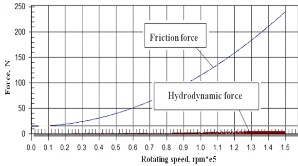
Figure 15 Forces acting on seal ring S4
