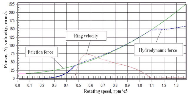
Figure 19 Forces acting on seal ring S8
