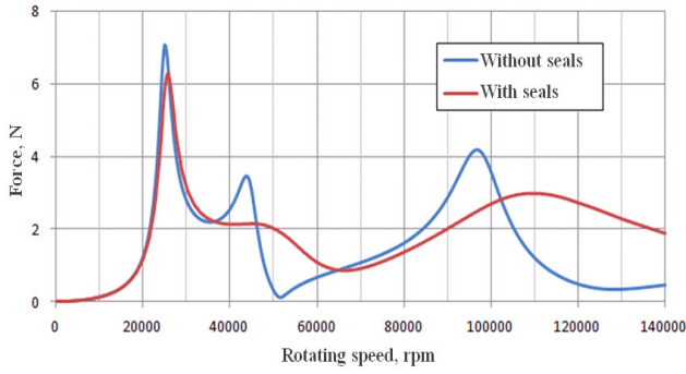
Figure 5. Loads in section elastic-damping support 1
