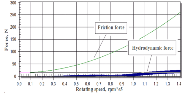
Figure 12 Forces acting on seal ring S5
