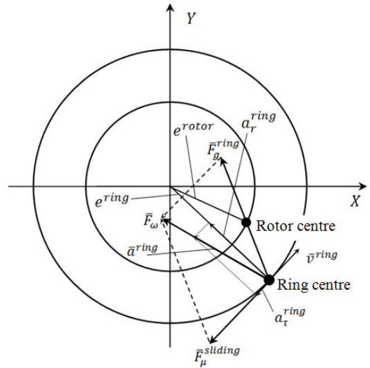
Figure 10. Vector scheme of ring motion
