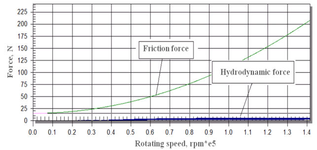
Figure 13 Forces acting on seal ring S8
