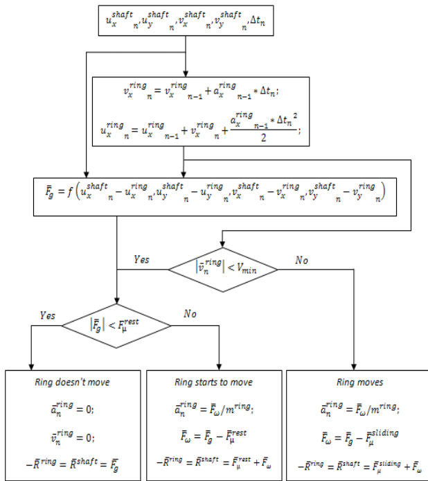
Figure 9. Flow chart of algorithm for determination of seal reaction
