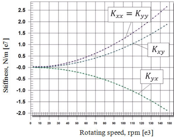
Figure 3. Stiffness coefficients of S4 seal
