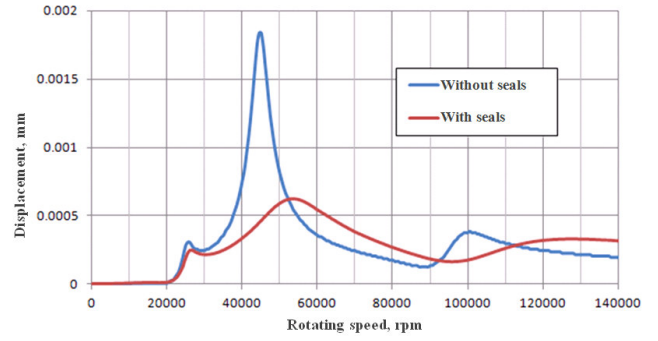
Figure 8. Displacement in section 1 of pump stage
