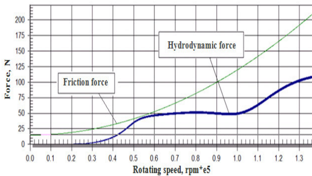
Figure 17 Forces acting on seal ring S6
