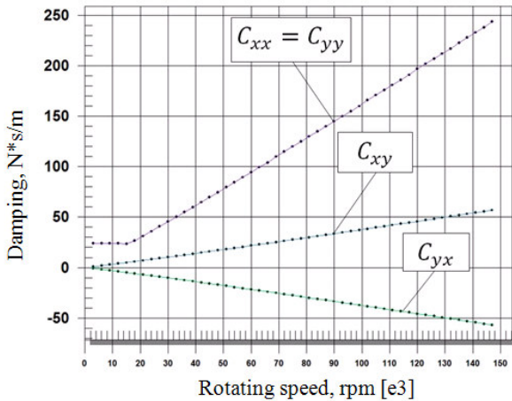
Figure 4. Damping coefficients of S4 seal
