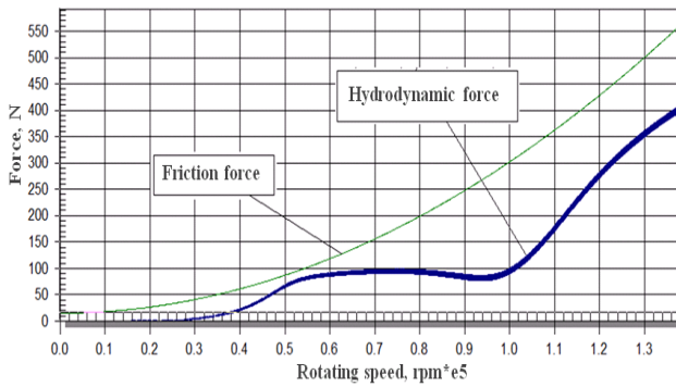
Figure 16 Forces acting on seal ring S5
