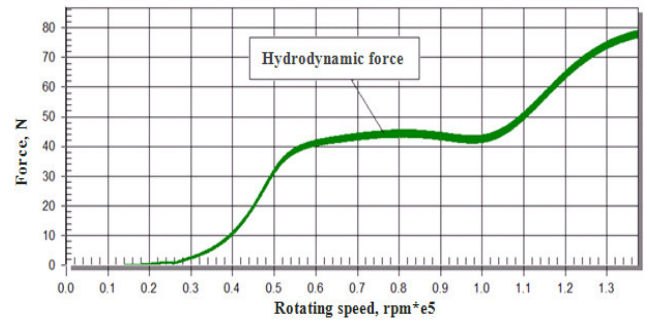
Figure 18 Hydrodynamic force in annular seal S7 (without ring)
